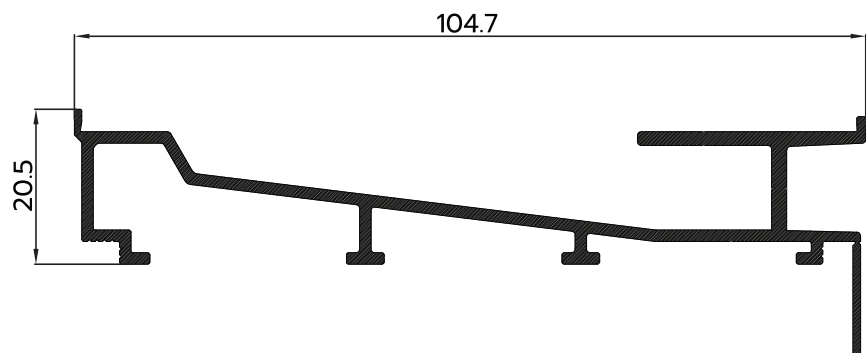
P-003399 Subsills
