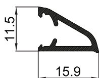
P-003301 Headsill
